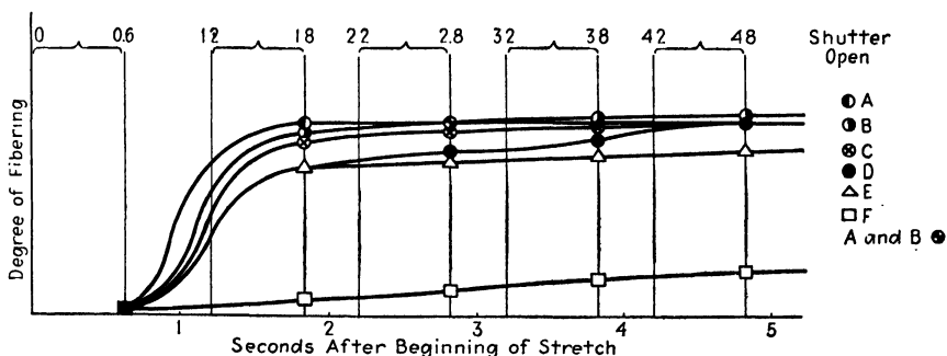
FIG. 2.—Time lag of fibering at different temperatures. A. Temperature, 15°C. Time of relaxation, 0.6 sec. B. Temperature, 15°C. Time of relaxation, 2.0 sec. C. Temperature, 25°C. Time of relaxation, 0.6 sec. D. Temperature, 27°C. Time of relaxation, 0.6 sec. E. Temperature, 30°C. Time of relaxation, 0.6 sec. F. Temperature, 35°C. Time of relaxation, 0.6 sec.
